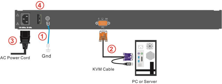
1-4 cable connection
