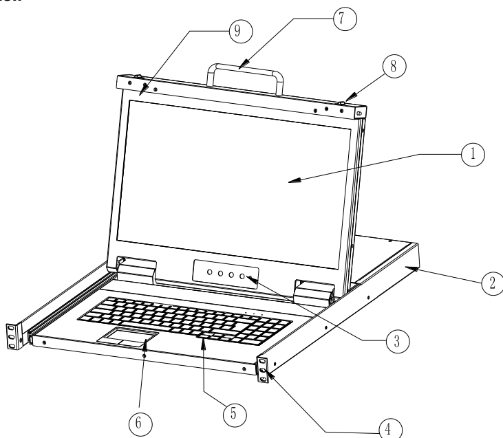
1-2 front view
